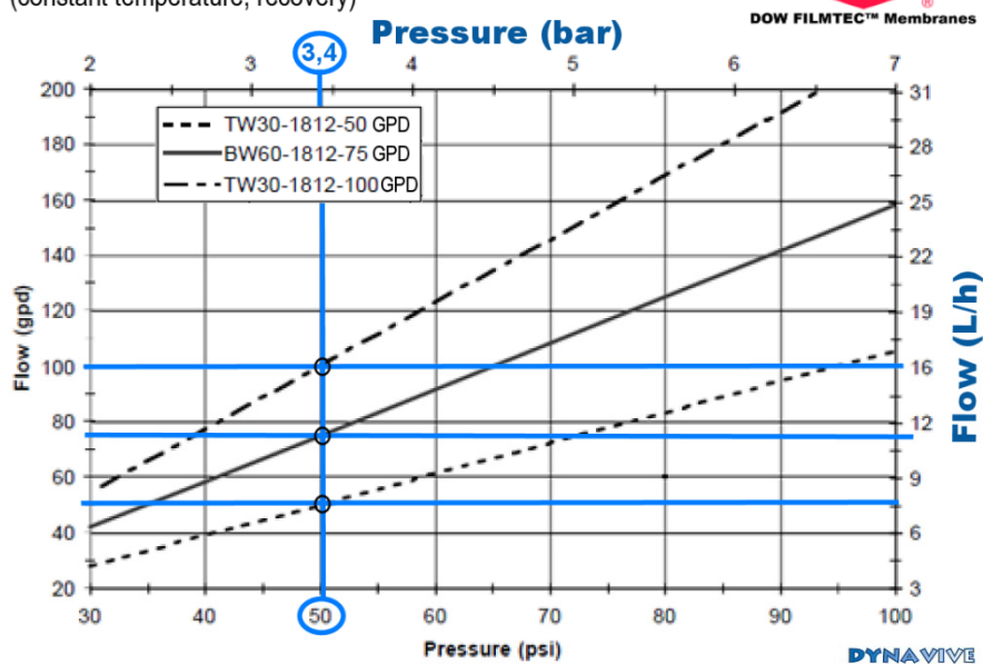
Impact of pressure on permeate flow (constant temperature, recovery)
