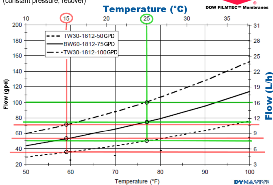
Impact of temperature on permeate flow (constant pressure, recover)
